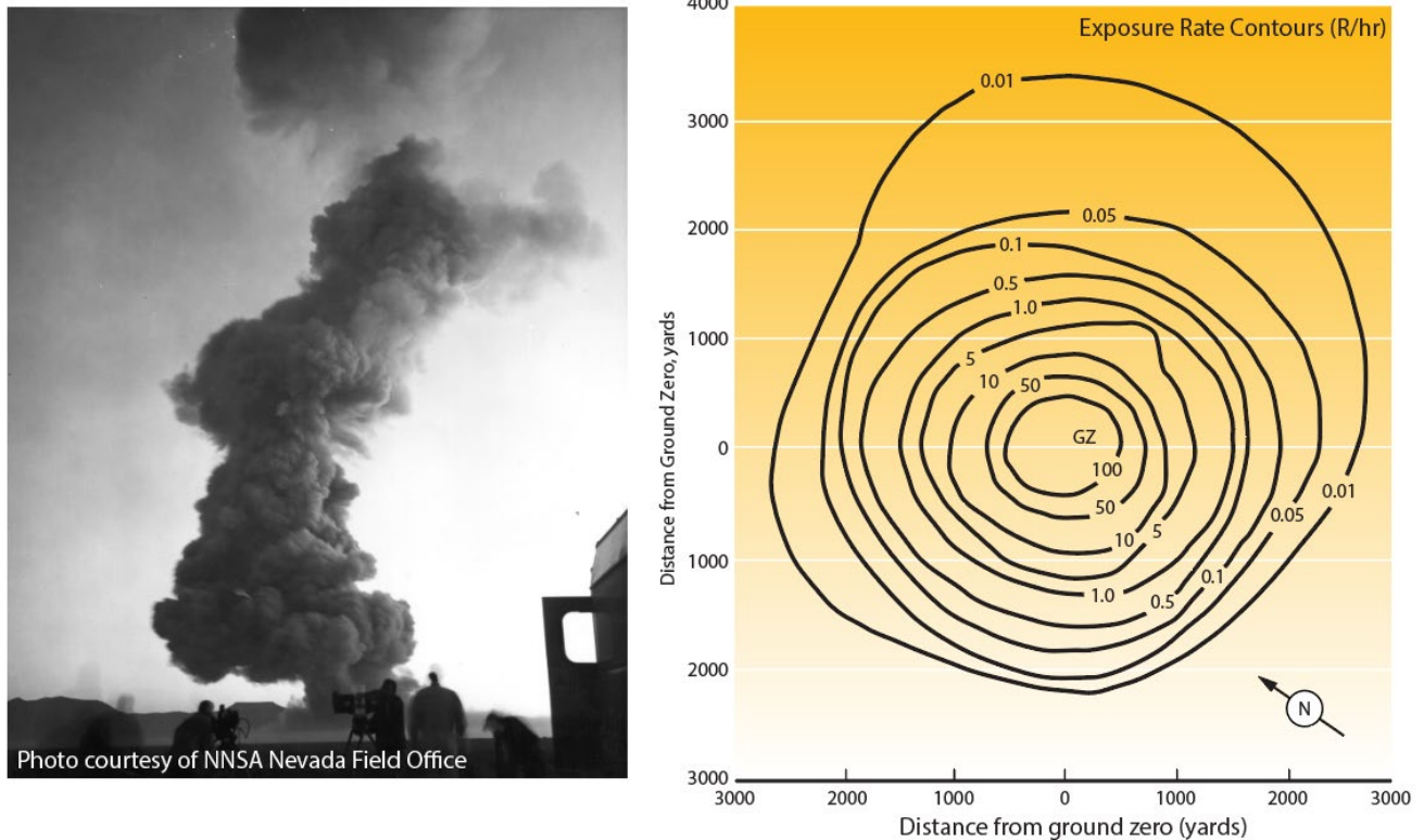
Figure 9: (Left panel) The 74 kT Plumbbob - Hood test was detonated at 1500' on July 5, 1957. (Right panel) Map of exposure rates (R/hr) one hour after detonation around ground zero (GZ).
